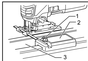
1. Screw 2. Guide rail adapter 3. Guide rail
