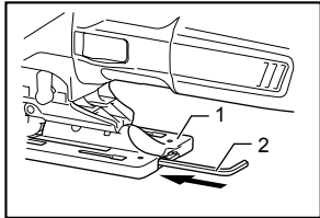
1. Base 2. Hex wrench
