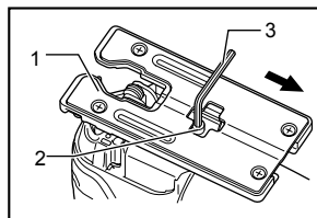
1. Base 2. Bolt 3. Hex wrench
